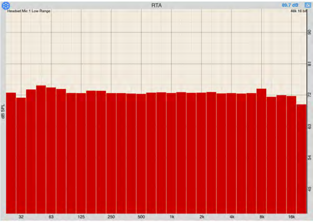
After Algorithm
