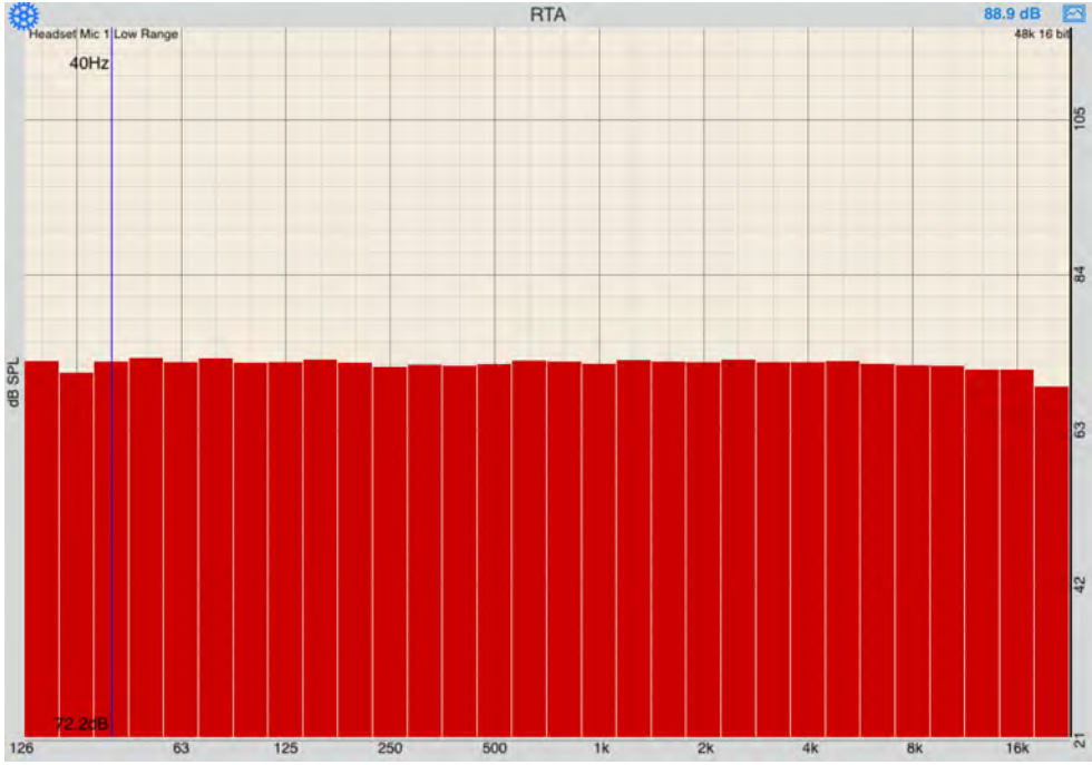
After Algorithm
