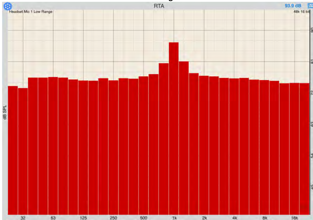
Before Algorithm
