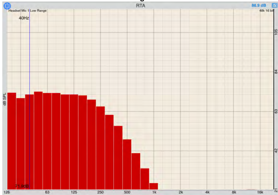
After Algorithm
