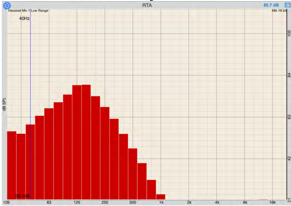
Before Algorithm
