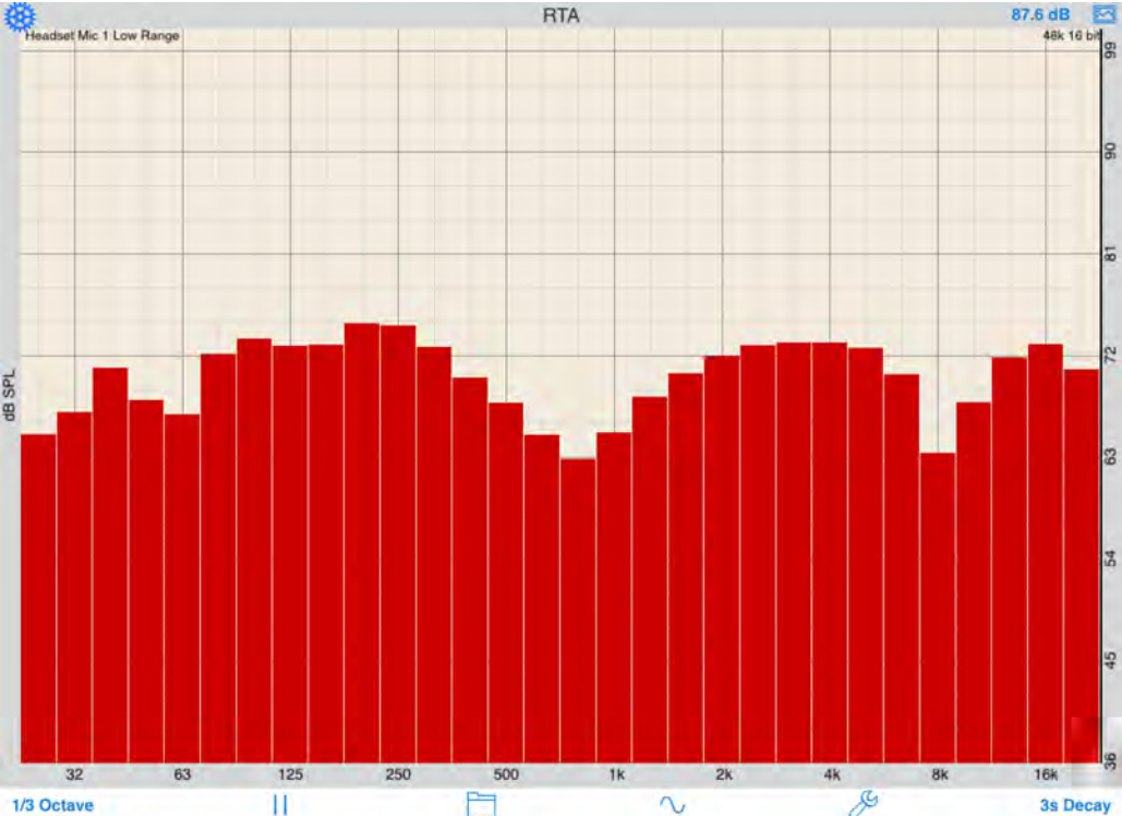
Before Algorithm
