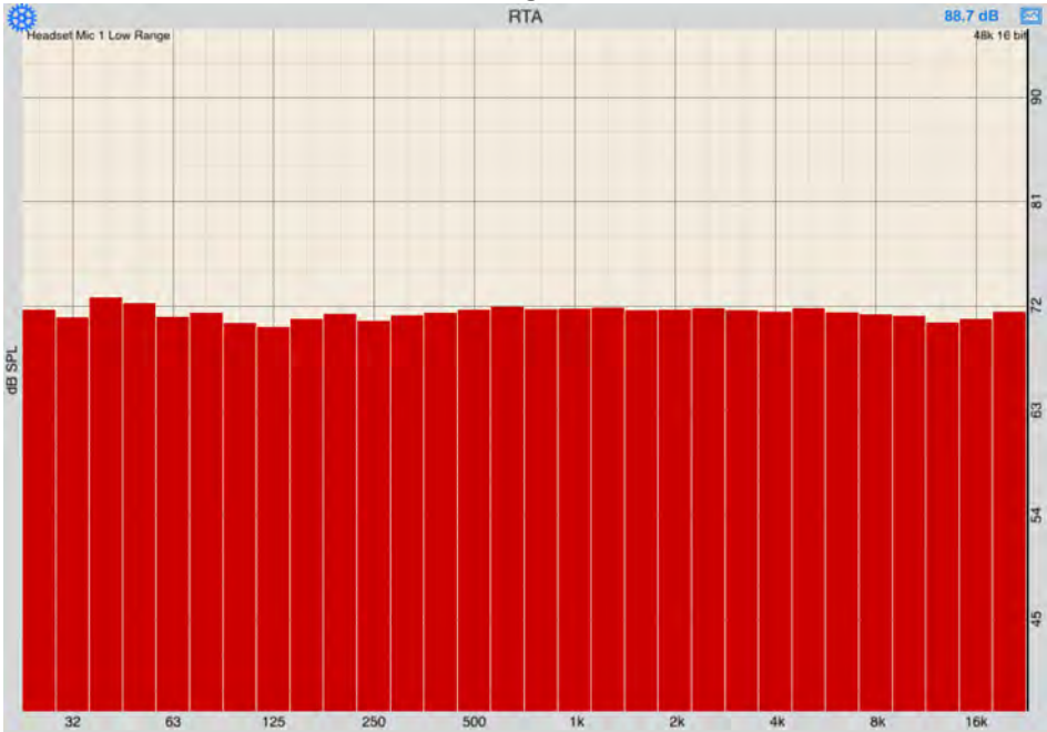
After Algorithm
