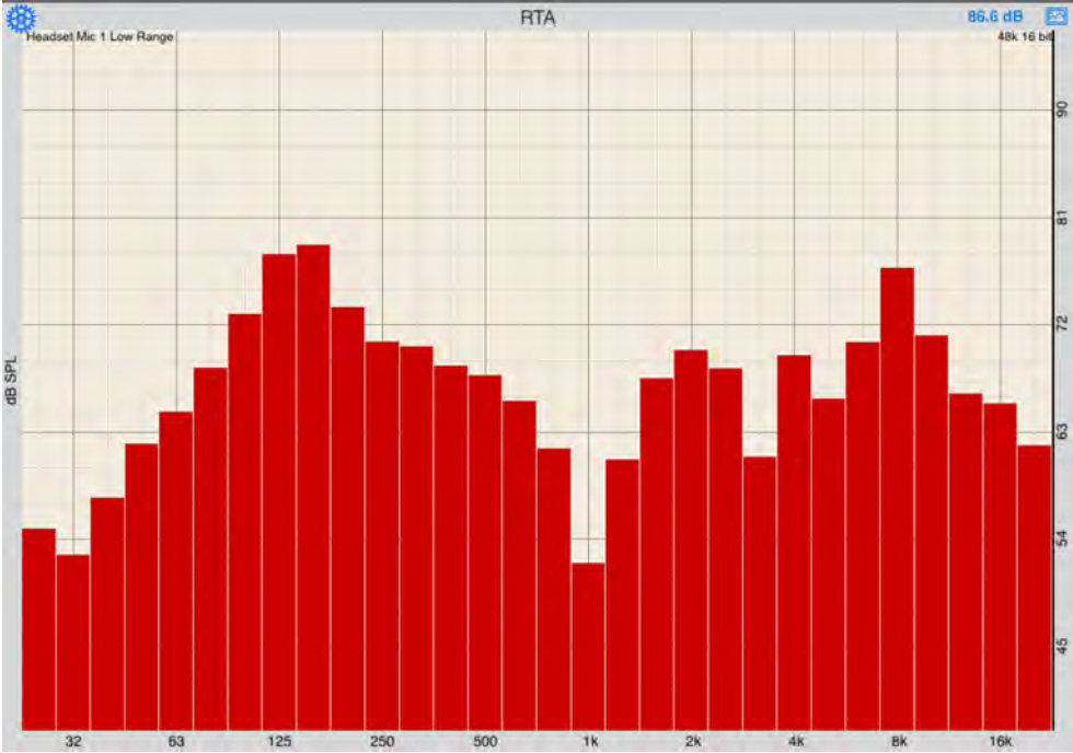
Before Algorithm
