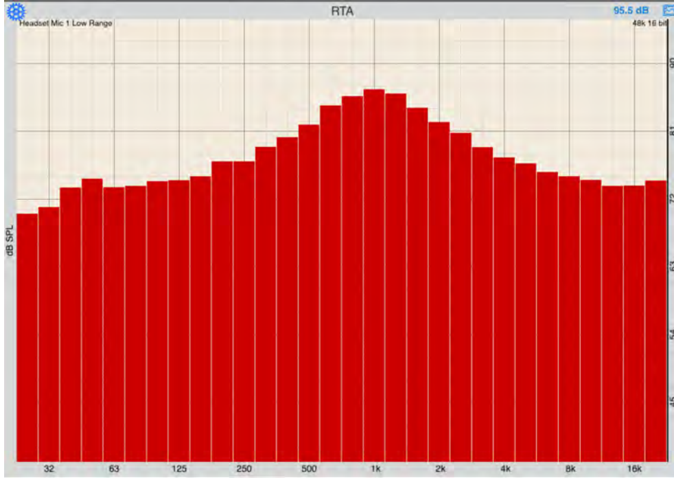
Before Algorithm
